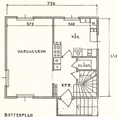
BOTTENPLAN
