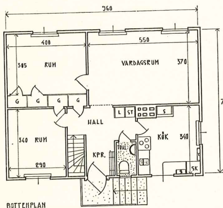
BOTTENPLAN
